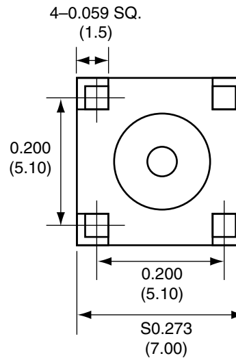
BACK VIEW
