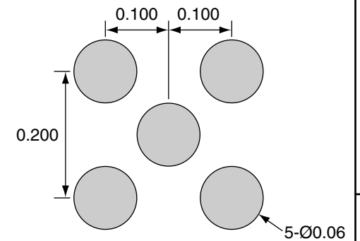
RECOMMENDED FOOTPRINT
